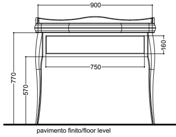
7363 Mobile cassetto laccato nero lucido per lavabo 100 Bright-black draw unit for washbasin 100 lacquer finish
