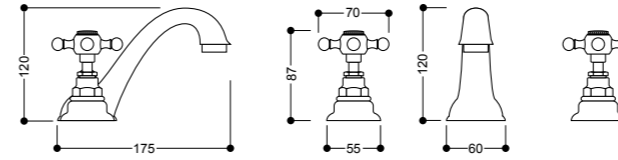
7391 Batteria lavabo 3 fori s. a. Three holes basin mixer with pop up waste
