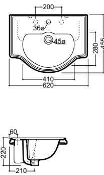
1030 Lavabo incasso 62x46 monoforo (tre fori a richiesta) One hole inset basin 62x46 (three holes on demand)
